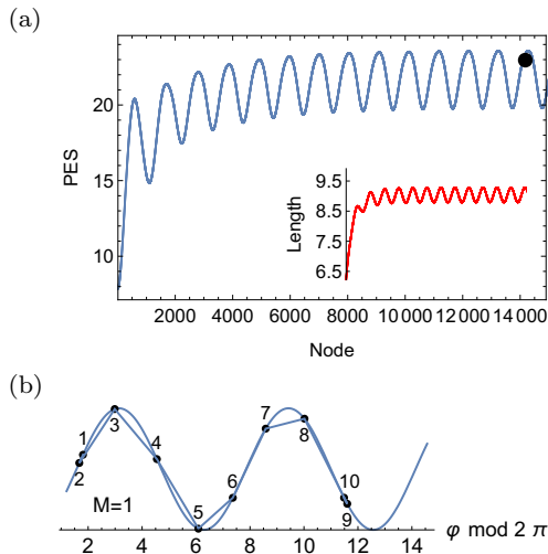
Fig. 15 (a) Langevin profile (PES only) for a non unique excitation, see text. The red inlay is the changing of the length of the chain under the 'downhill' sliding with this force. The black bullet in the upper right corner is a possible entry point to a 'wormhole' to M=2 . Its structure is given in panel (b).
