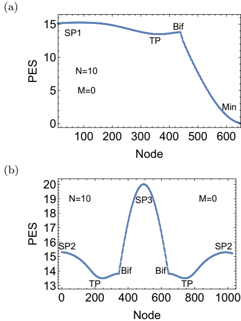
Fig. 5 Energy profiles of NTs from SP_1 (a) and from SP_2 (b) for M=0 . The search direction is the unitary one. Both NTs bifurcate at a VRI point.
