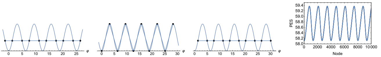
Fig. 22 Minimum left, SP_1 centre left, and second minimum centre right, of the FK chain with M=5 fluxons. Both minimums have the same energy, but a different length. There exists a mirror symmetric SP (not shown). The right panel is the energy profile over the MEP through minimums and SP_1 calculated by a Langevin equation with unitary direction (1, \dots, 1) .
