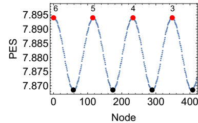
Fig. 2 Energy profile over a piece of the MEP through minimums (black) and SP_1 (red) of Fig. 1 calculated by a Newton trajectory (NT) [2] to a unitary direction (1, \dots, 1) . On the theory of NTs see part II. The numbers over the SP s depict the consecutive \phi_k which cross the SP . Note the very low energy difference of the two stationary points. Thus, the pathway is nearly flat, and the critical current is very low.
