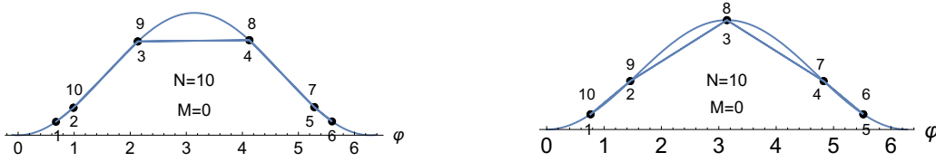
Fig. 4 Extended SP_1 (left) and SP_2 (right) for M=0 . The left numbering of the PDs goes from 1 to 6 with increasing value, but then back. So that \phi_{6+k} = \phi_{6-k} , k = 1, \dots, 4 where for the right hand case it goes up to i = 5 and then symmetrically back. Besides the foldings, the structures look like the minimum and the SP_1 of the M = 1 -case in Fig. 1.
