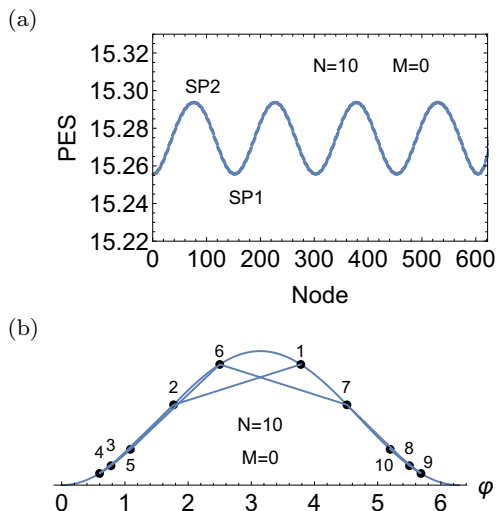
Fig. 6 (a) Energy profile over a piece of an NT through consecutive SP_1 and SP_2 , for M=0 . The search direction of the NT is the first positive eigenvector of SP_1 . The NT balances on a ridge. (b) A stroboscopic structure at the end of the NT: the PDs are 'rotated' where the chain stays on the place. Compare the order in Fig. 4.
