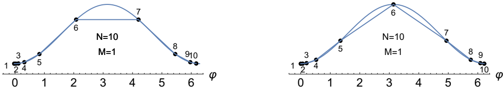
Fig. 1 Equilibrium structures (minimum left and SP_1 right [17,20]) of the FK chain with N=10 PDs under the ring condition (5) with M=1 . The bullets are artificially lifted on the potential to guide the eye. Because we use a_0 = 0 in the model potential (4), the PDs can form 'nearly together lying clouds' in the minima of the cosine function.
