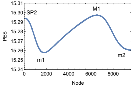
Fig. 10 Energy profile (PES only) over a Langevin solution starting at SP_2 , for M=0 . The bias direction is the first positive eigenvector of SP_1 , \mathbf{l}_{rot} of Fig. 6. The excitation amount is F_{dc} = 0.1 , but the step length of t -steps is 0.01. After step 15000 it descends to the global minimum (not shown). M1, m1, and m2 are maximal and minimal TPs.
