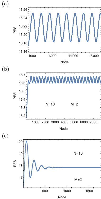
Fig. 19 Energy profile of three dc-driven Langevin solutions in case M = 2 on the PES only (without representation of the tilting) for N = 10 PDs. (a) for F_{dc} = 0.15 with the start in a minimum, (b) for F_{dc} = 1 , and (c) for F_{dc} = 7.5 . We find a stable small vibration in cases (a) and (b) after an initial settling. In case (c) the curve flattens out quite analogously to the case M = 1 . Note the different t -scales in the three panels.
