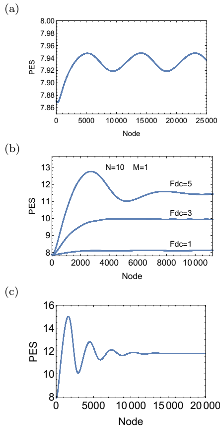
Fig. 12 Energy profile of dc-driven Langevin solutions on the PES only (without representation of the tilting, compare parts I and II [1,2]) for N = 10, M = 1 and direction (1, \dots, 1) . (a) for F_{dc} = 0.15 , somewhat over the critical force F_c = 0.02542 , with the start in a minimum, (b) the profiles for F_{dc} = 1, 3 , and 5 , (c) for F_{dc} = 7.5 . We find a stable small vibration in cases (a) and (b) after an initial settling. In case (c) the curve flattens out.
