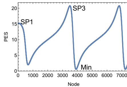
Fig. 7 Energy profile over a Langevin solution on the PES only (without representation of the tilting, compare parts I and II [1,2]) starting at SP_1 , for M=0 . The excitation direction is the unique case, (1,1,\dots,1) , and the amount, F_{dc} = 3.5 is a bit over the critical force, F_c = \sqrt{10} = 3.16 . After settling in the first cycle, the solution alternately crosses the regions of the minimum and of the SP_3 .
