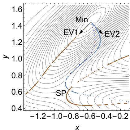
Figure 5: MB surface 18 with modified SEGO curves to the dyadic matrix \mathbf{D} , see text. The brown curve is to direction of the first eigenvector along the valley floor of the global minimum. The blue curve starts with eigenvector 2. For comparison the points of Fig. 1 are included.
