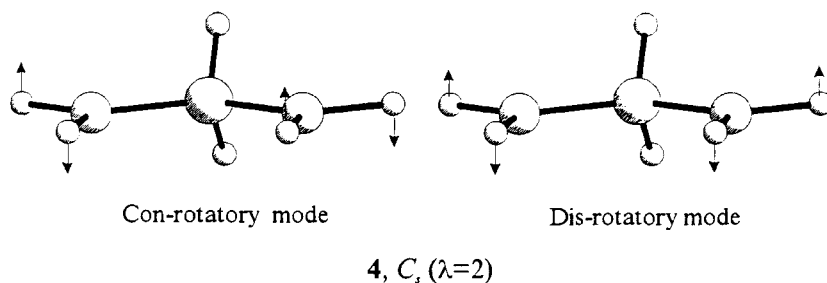
FIGURE 5. The shape of the conrotation [ \nu(A_2) = 119.8 \text{ cm}^{-1} ] and the disrotatory [ \nu(B_1) = 325.3 \text{ cm}^{-1} ] modes corresponding to the two imaginary frequencies of 4 . Arrows denote the components of the corresponding mode.
