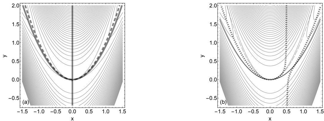
FIG. 1. GO surface with flat saddle at (0,0) . (a) The fat curve is the NT were the x -component of the gradient is zero, it bifurcates at the VRI point. The fat-dashed curve is the NT were the y -component of the gradient is zero. (b) The NT to direction y=-x (fat squares) falls apart to two pieces. If one starts anywhere on the right piece one avoids the singular point. The full parabola is a set of points with zero eigenvalues of V_{GO} . The thin dashed parabola is the border between the ridge and the valleys.
